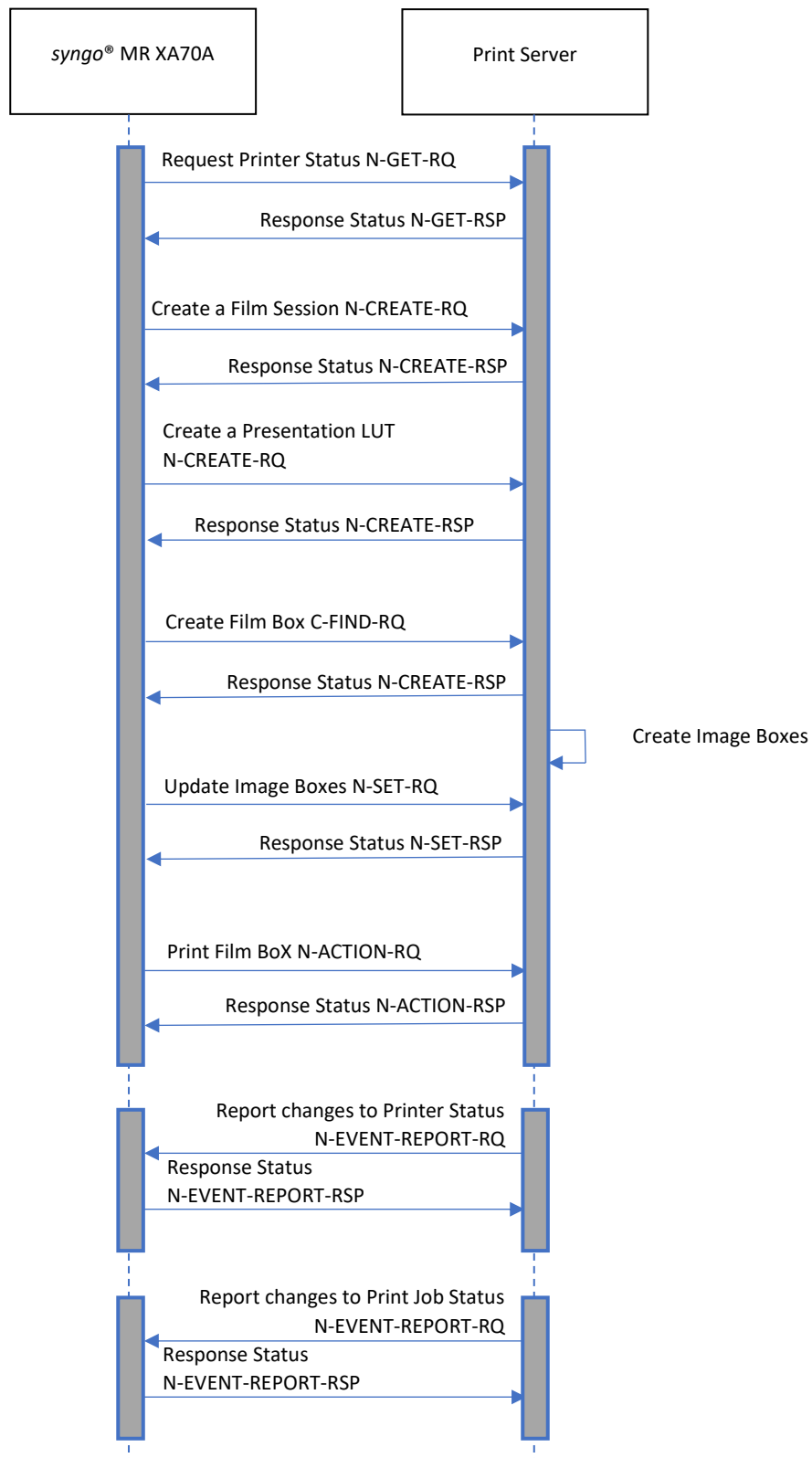
Figure 4: Sequence Diagram for Real World Activities - Printing
