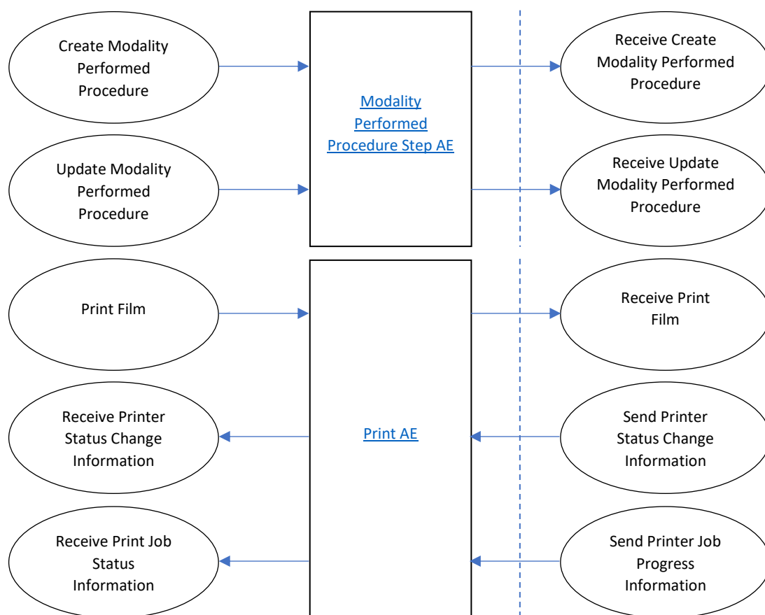
Figure 1: syngo® MR XA70A DICOM Data Flow diagram – Acquisition Workflow
