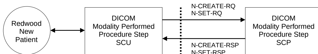
Figure 6. MPPS Model
