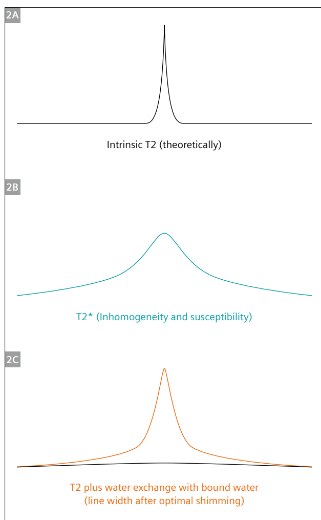
2 The figure depicts the linewidth to which the water signal is shimmed – (2A) theoretical FWHM that equals 1/(\pi T_2) , (2B) significantly broadened linewidth with inhomogeneities and susceptibility effect with a patient inside the magnet, (2C) Result after shimming. Two water signals (free water and bound water) are shown in slow exchange. They are chemically indistinguishable but with different rotational and translational energies, and thus different T_2 .
