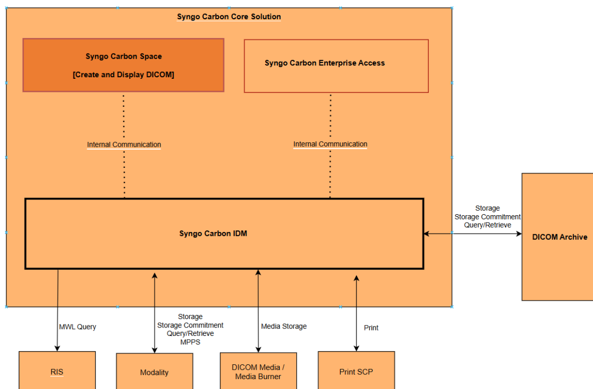
Figure 1: Overview of Implemented Services
